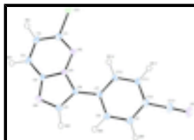
Fig. 1. , The ORTEP view of the title compound with 50% probability displacement ellipsoids for non-H atoms.
